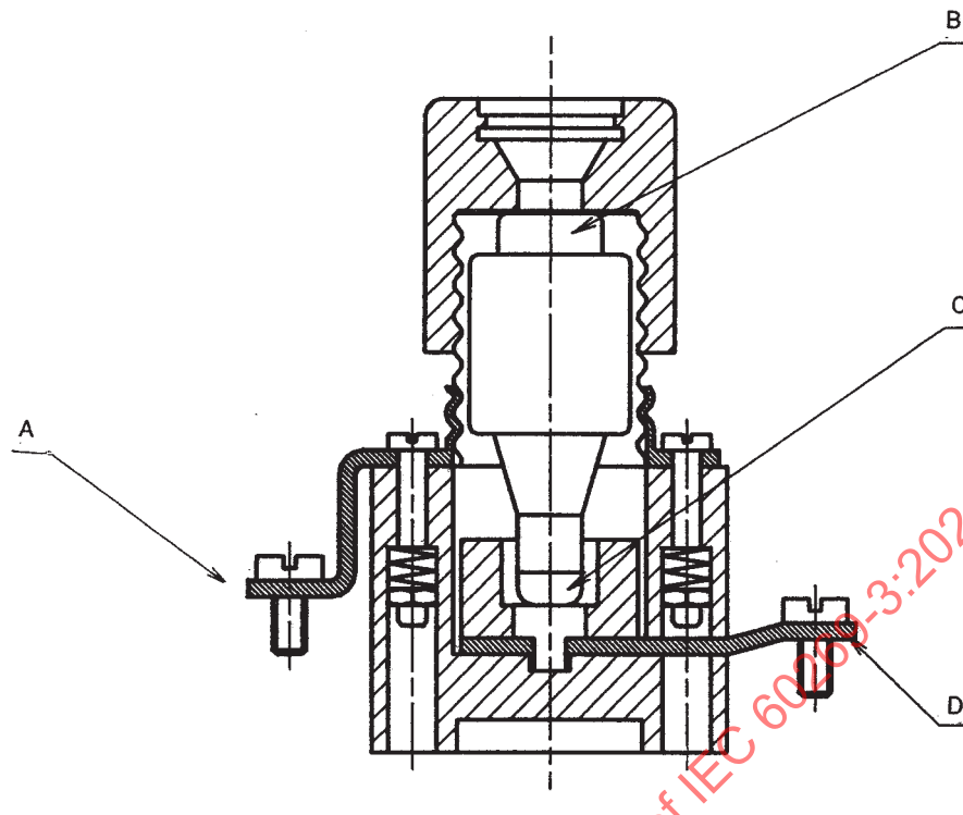
Figure 109 – Measuring points according to 8.3.3, 8.3.4.1 and 8.10.2 of fuse system A
