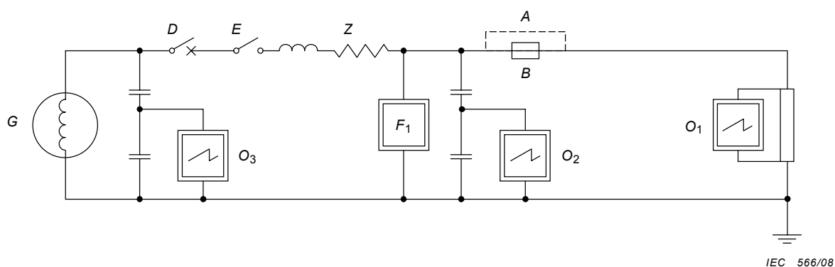
Figure 3a – Test duties 1, 2 and 3
