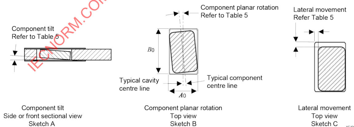
Figure 4 – Maximum component tilt, rotation and lateral movement
