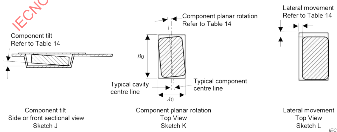
Figure 13 – Maximum component tilt, rotation and lateral movement
