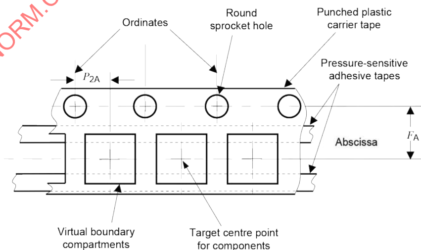
Figure 24 – Type 4 coordinate system
