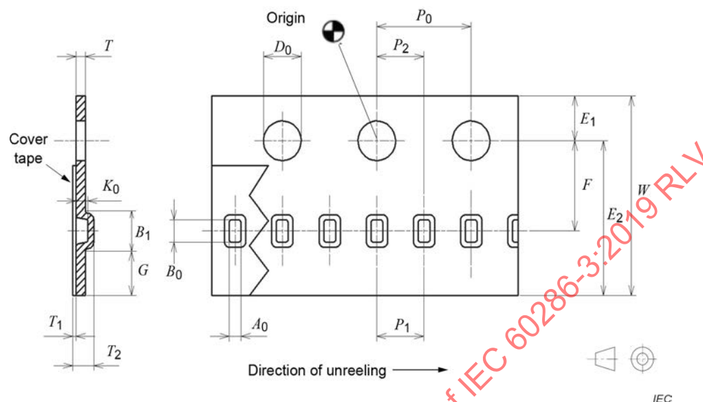
Figure 11 – Type 2b carrier tape
