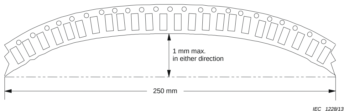
Figure 21 – Camber (top-view)
