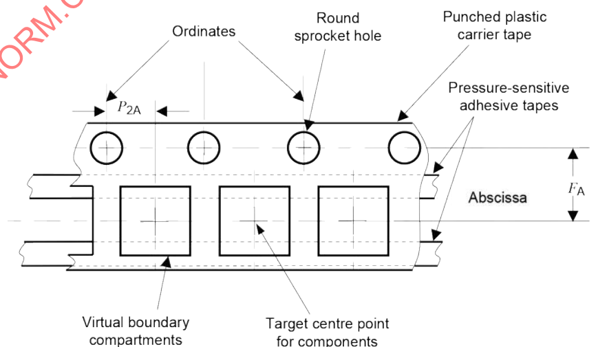
Figure 24 – Type 4 coordinate system
