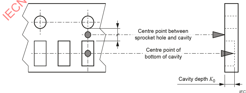
Figure A.3 – Cavity depth dimension
