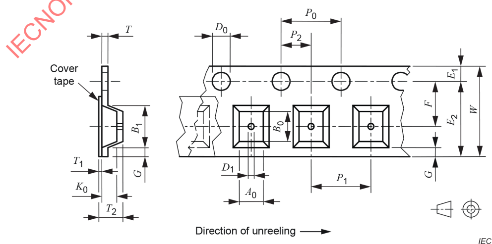
Figure 8 – Blister carrier tape dimensions (8 mm, 12 mm, 16 mm and 24 mm)
