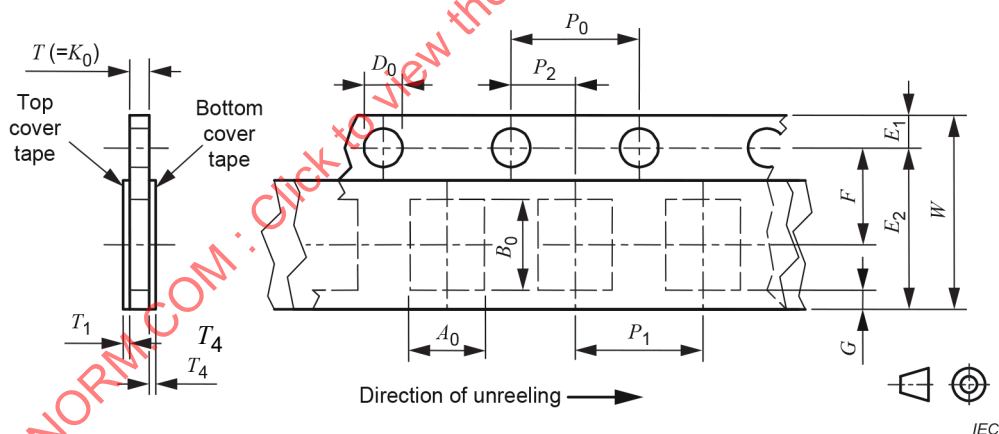
Figure 2 – 8 mm and 12 mm punched carrier-tape dimensions (4 mm cavity pitch)
