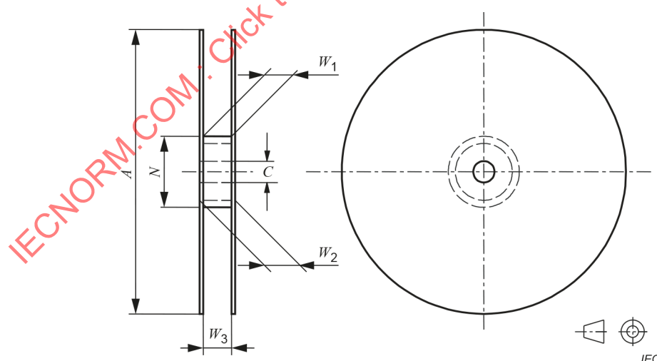
Figure 26 – Reel
