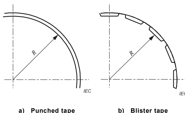
Figure 21 – Bending radius
