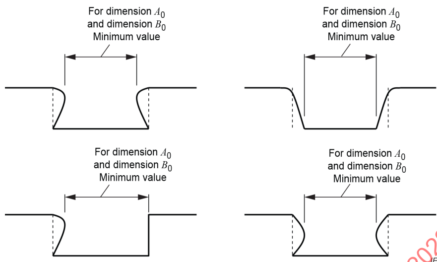
Figure A.2 – Cavity cross-section
