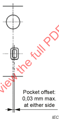
Figure 12 – Maximum pocket offset
