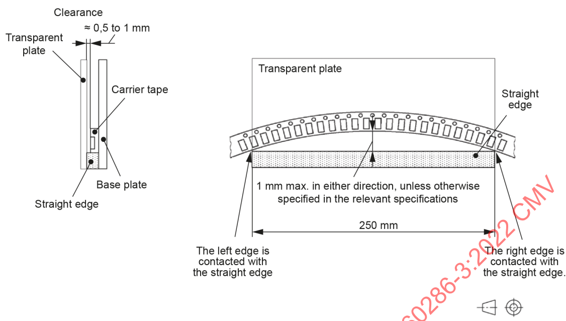
Figure 22 – Measuring method and camber
