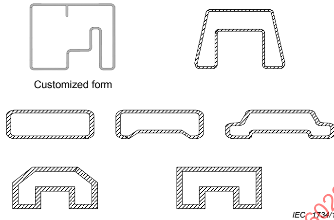
Figure 1 – Shape and cross-sections of stick magazines
