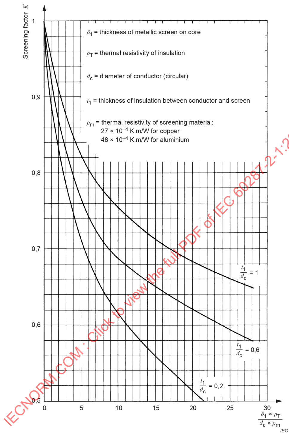
Figure 4 – Thermal resistance of three-core screened cables with circular conductors compared to that of a corresponding unscreened cable (see 4.1.2.3.1)
