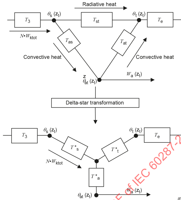
Figure B.1 – Delta-star transformation
