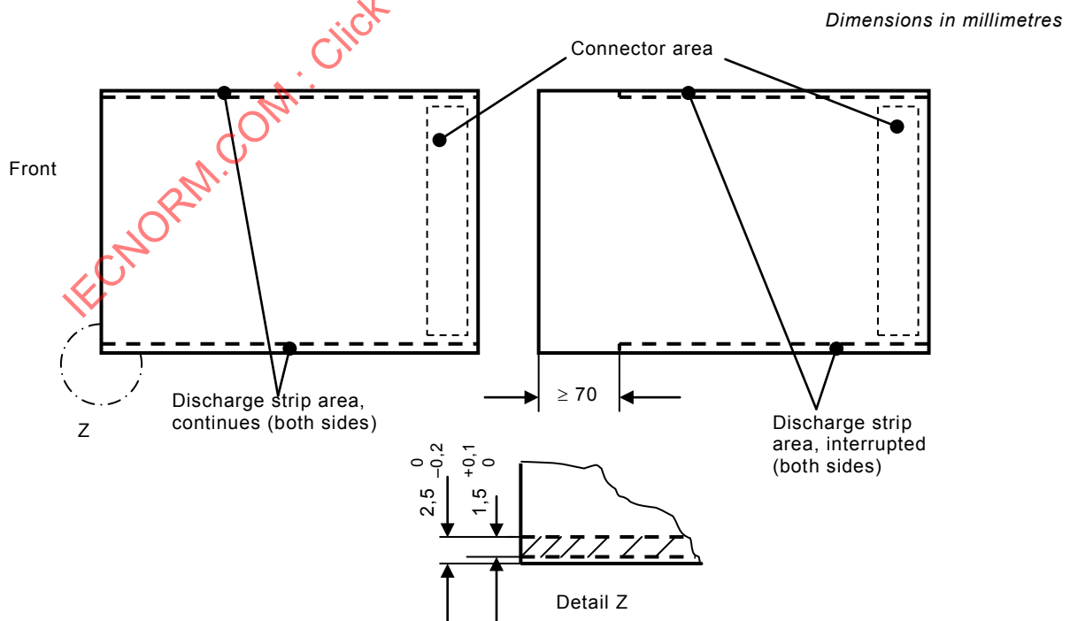
Figure 17 – ESD strip interface dimensions
