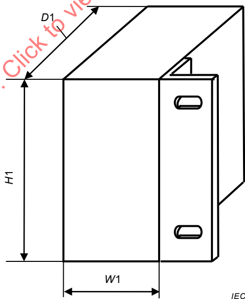
Figure C.3 – Type C: Vertical flange mounting
