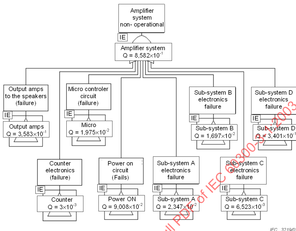
Figure A.2 – Fault tree for an audio amplifier
