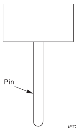
Figure 4 – Gauge for verification of the minimum withdrawal force
