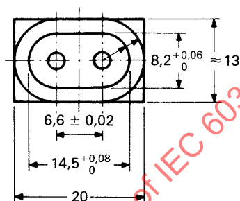
Figure 2 – "GO" gauge for connectors according to standard sheet C1
