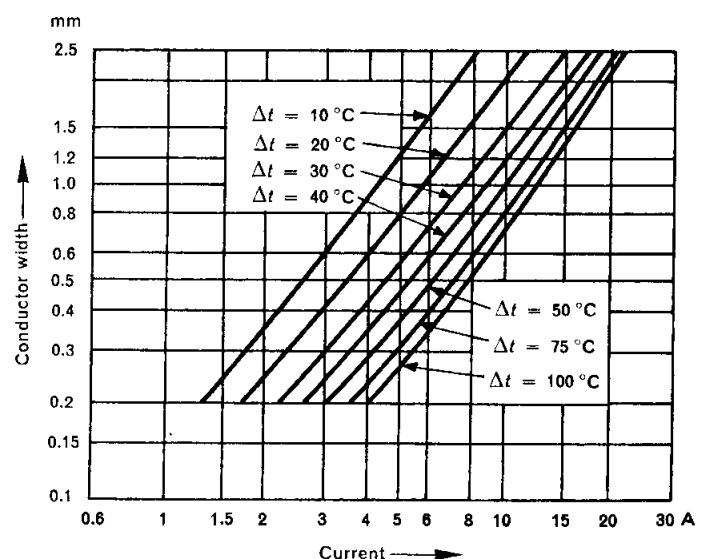
Conductor thickness 105 μm
