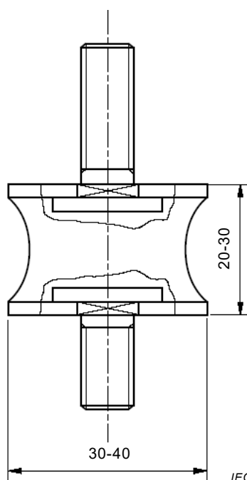
Figure 5 – Typical rubber bush for supporting the test ladder
