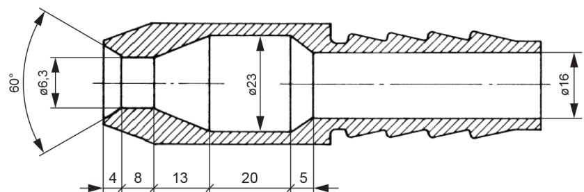
Figure C.3 – Hose nozzle
