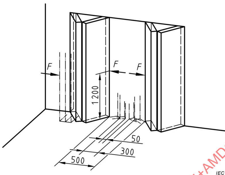
Figure II.3 – Folding doorset
