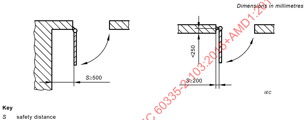
Figure CC.1 – Safety distances for opening movement of swing door
