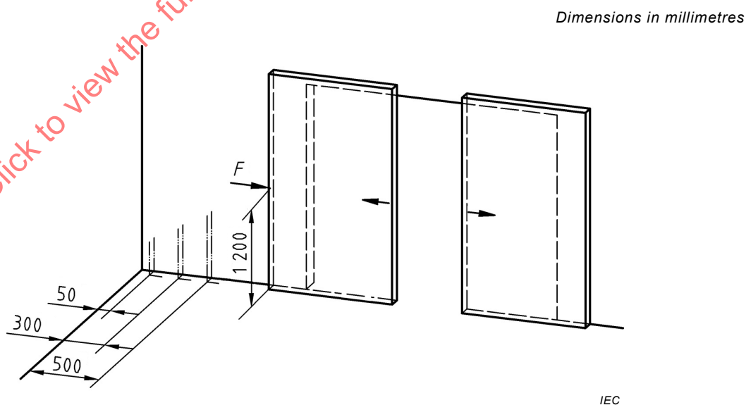
Figure II.2 – Double-leaf sliding doorset
