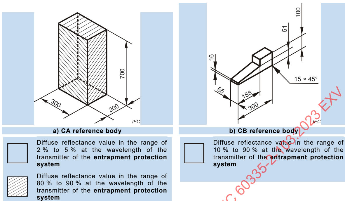
Figure FF.1 – Reference bodies
