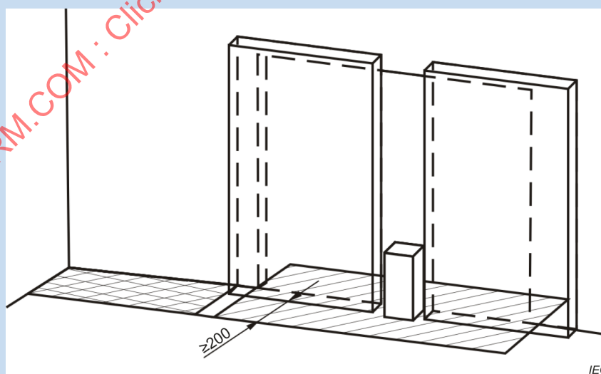
Figure EE.1 – Single-leaf sliding doorset
