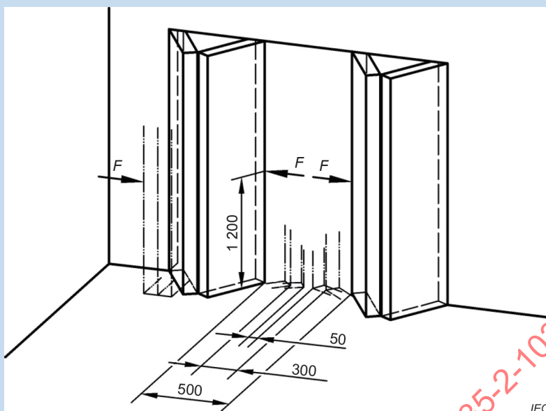
Figure II.3 – Folding doorset
