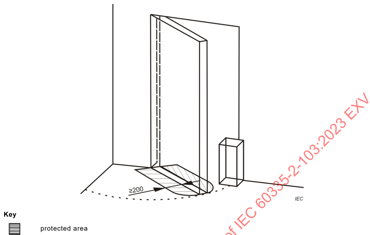
Figure EE.3 – Single-leaf swing doorset
