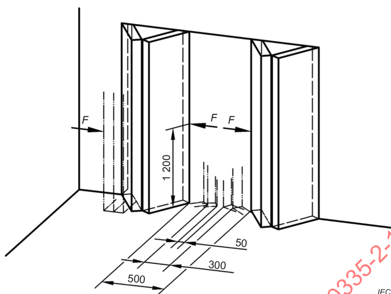
Figure II.3 – Folding doorset
