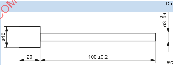
Figure 101 – Test rod for interlock concealment
