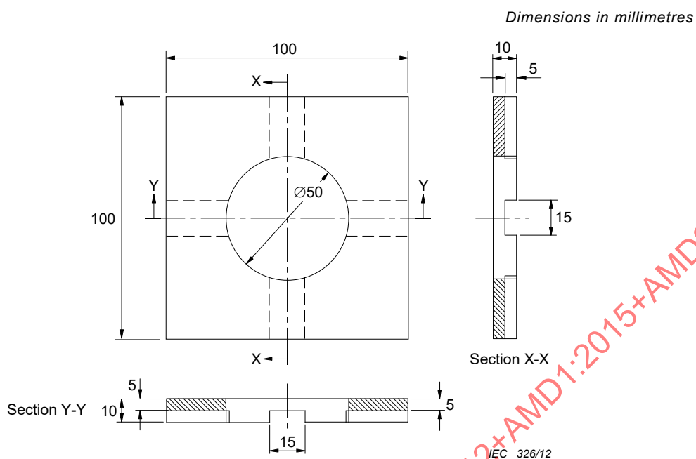
Figure 113a – Detail A – Lower part of mask
