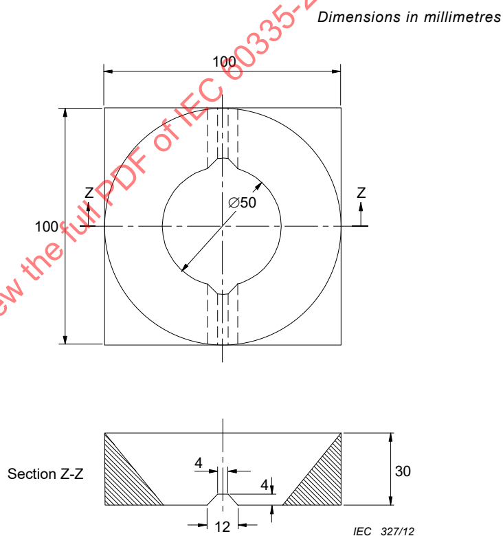
Figure 113b – Detail B – Upper part of mask
