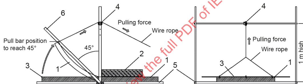
Example of guide pulley
