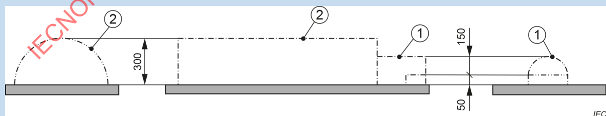
Figure 104 – Measuring points for appliances that are arranged over a person
