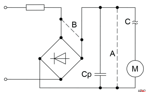
b) Series circuit
