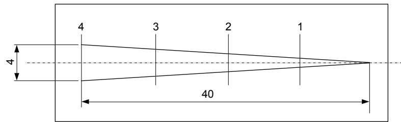
Figure GG.3 – Isosceles triangle arrow test gauge
