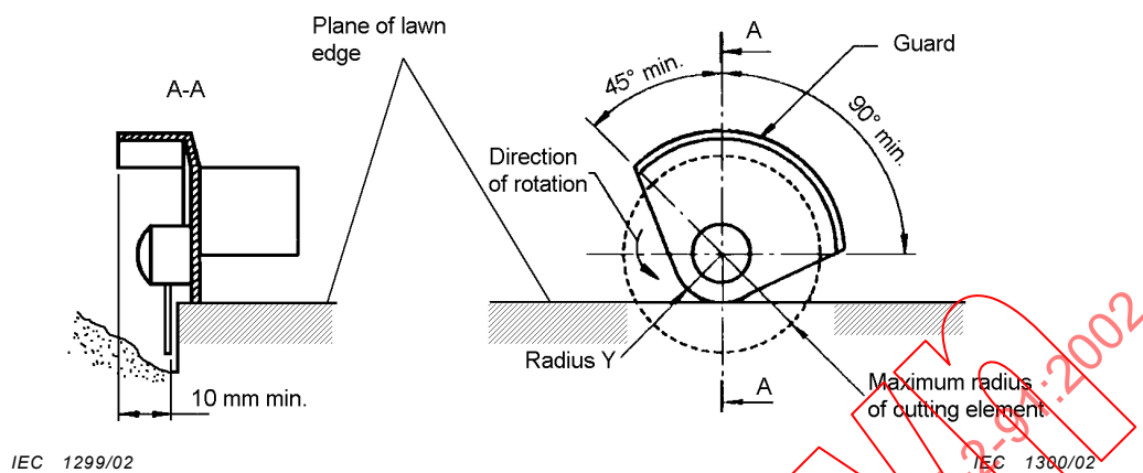
Figure 102a – View towards cutting means
