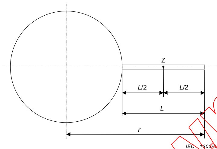
Figure 105a – Filament line
