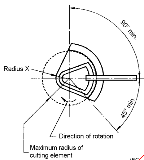
Figure 101a – Plane view
