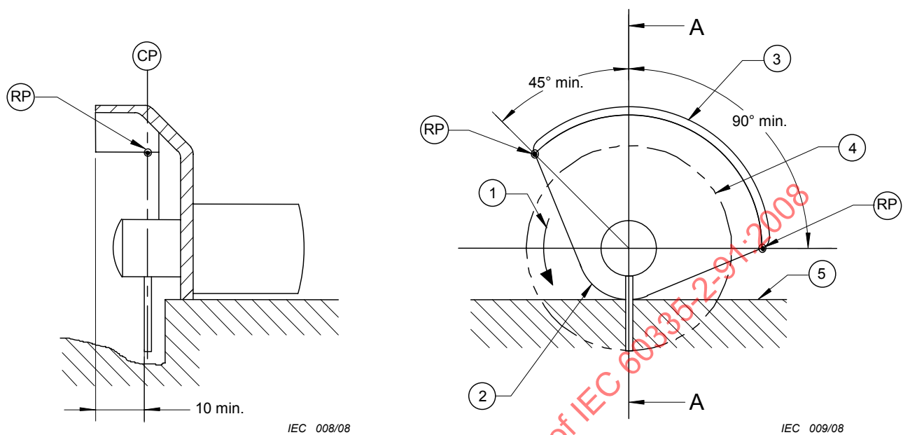
Figure 102a – Part section at AA (guard only)
