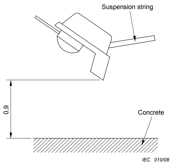
Figure 103 – Guard strength test (hand-held appliances)
