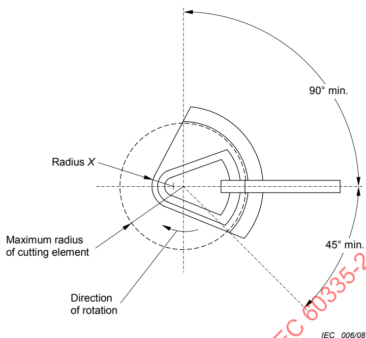
Figure 101a – Plan view
