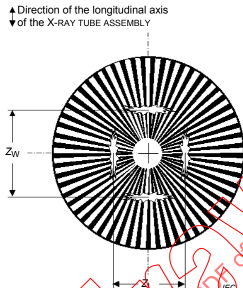
Figure 9 – Illustration of the zones of minimum modulation
