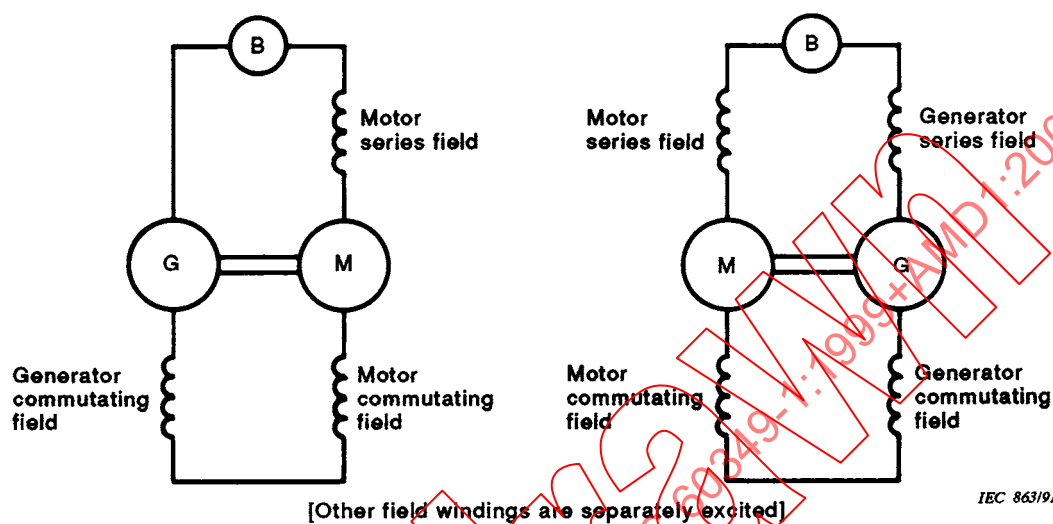
Figure B.2a – Motor test
