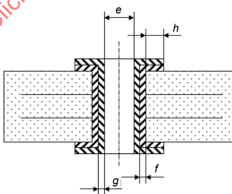
Figure 1 – Plated-through hole
