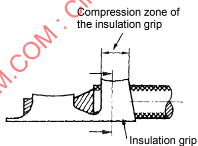
Figure 4c – Insulation grip
