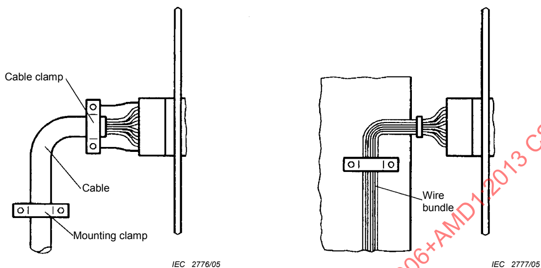
Figure 37 – Mounting of wire bundles/cables with crimped contacts
