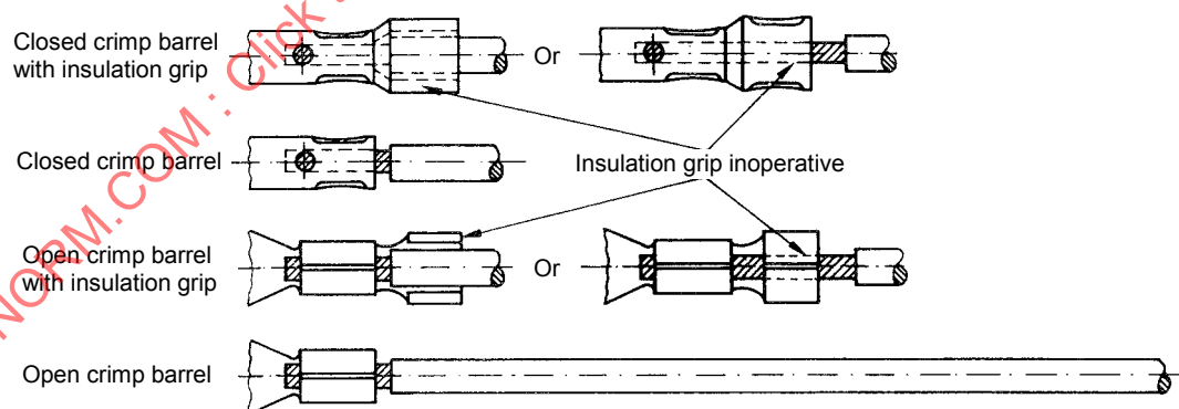
Figure 9 – Examples of type A specimens
