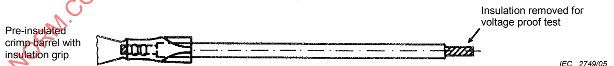
Figure 11 – Example of type C specimen
