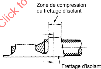
Figure 4c - Frettage d'isolant
