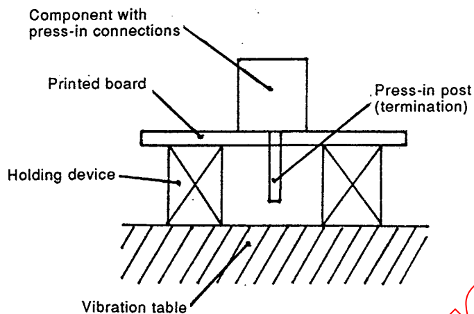
Figure 5 – Test arrangement, vibration
