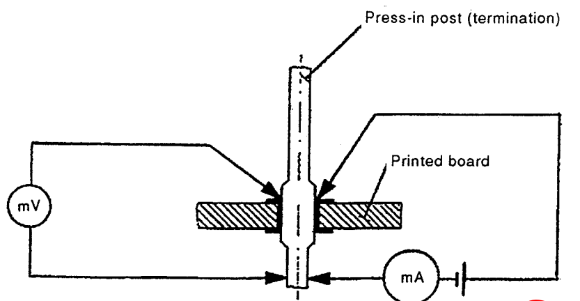
Figure 6 – Test arrangement, contact resistance
