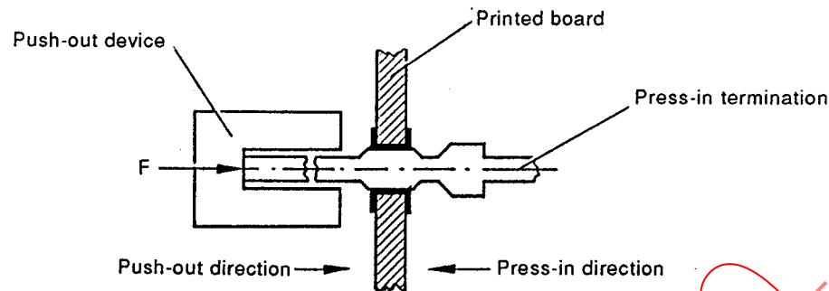
Figure 4 – Test arrangement, push-out force
