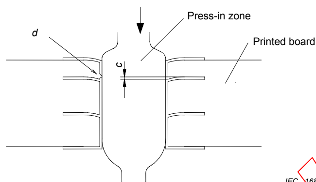
Figure 7 – Longitudinal section of a press-in connection
