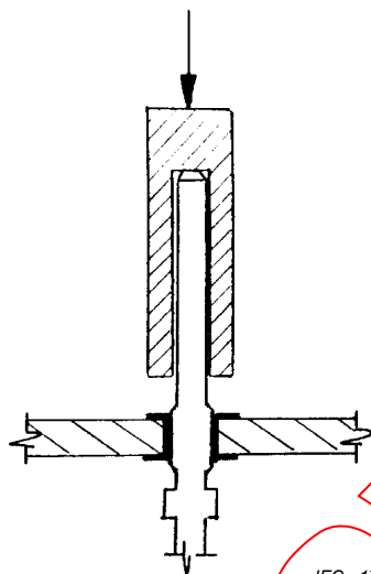
Figure A.1 – Example of a termination removal tool
