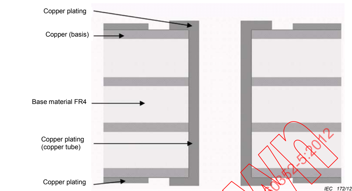
Figure A.2 – Conceptual composition of a four-layer printed circuit-board
