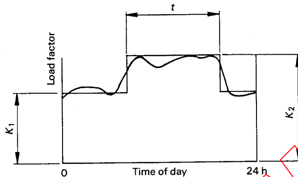
Figure 7 – Load cycle with peaks in close succession
