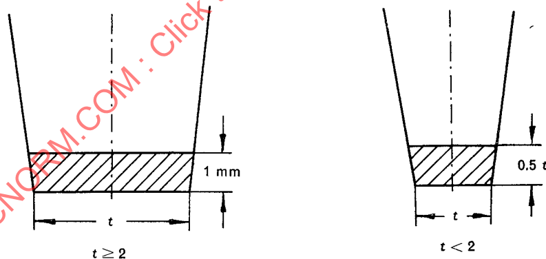
FIG. 5. — Tolerance on shape of the thin edge.
