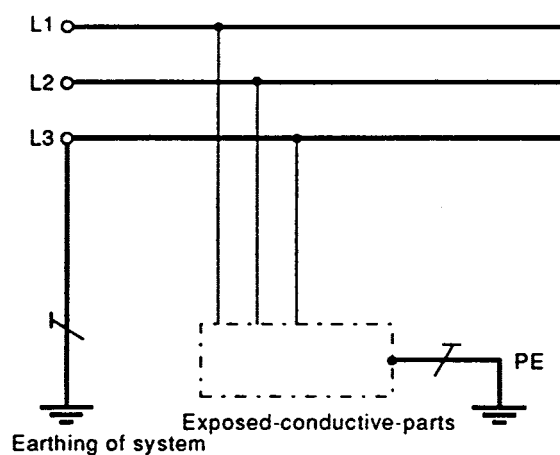
Figure 31D – TT system
