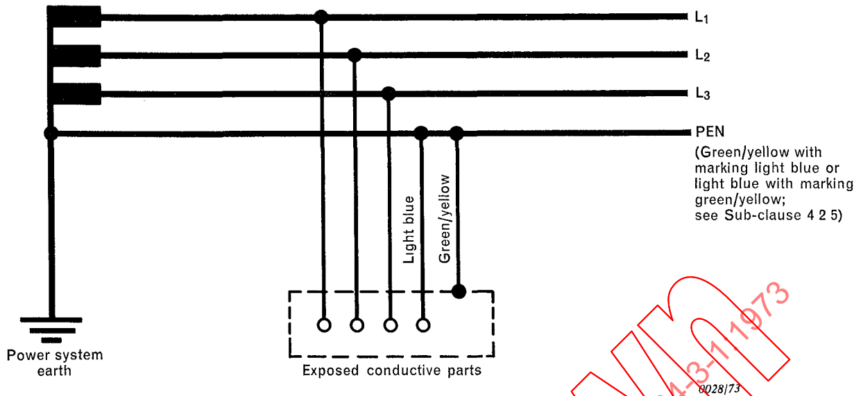
FIG 3 3 — Neutral and protective functions combined in a single conductor throughout system
