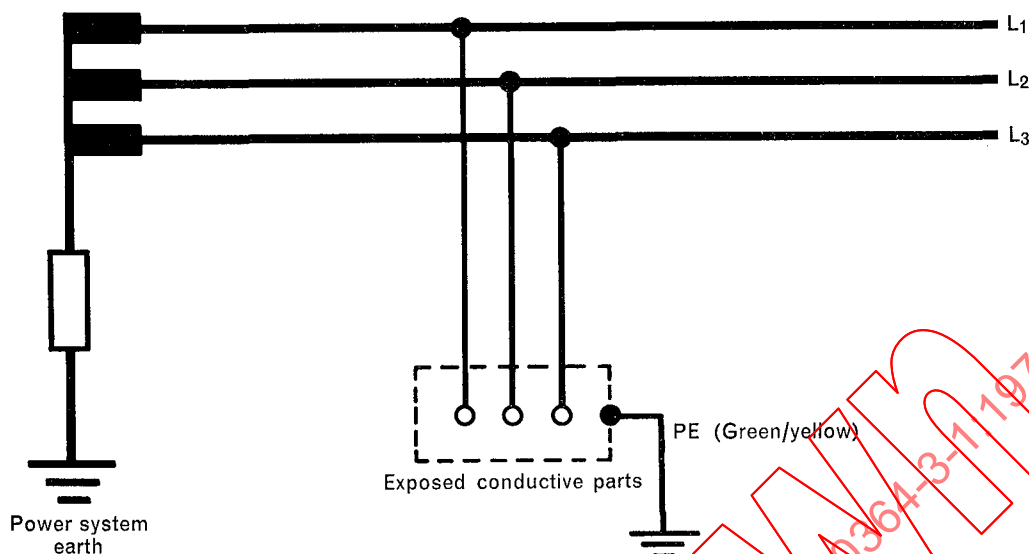
FIG 5 — Power system IT
