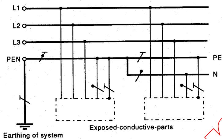
Figure 31B – TN-C-S system. Neutral and protective functions combined in a single conductor in a part of the system
