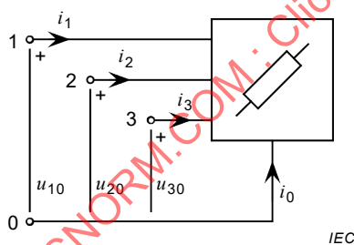
Figure 24a – Representation using that of Figure 3b for currents i and that of Figure 10a for voltages u
