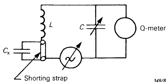
FIG. 6. — Schematic diagram of the measuring circuit.
