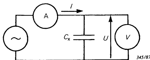
FIG. 1. — Schematic diagram of the measuring circuit.
