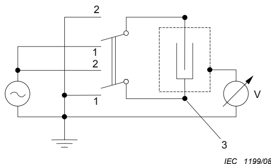
Three outer foil terminations
