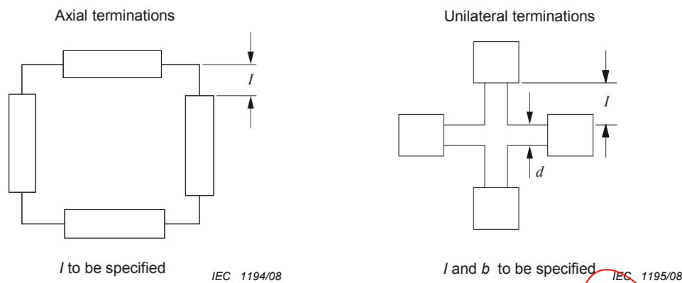
Figure 5 – Capacitor mounting arrangement
