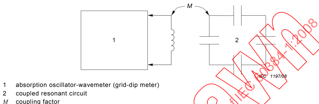
Figure 7 – Typical diagram of an absorption oscillator-wavemeter
