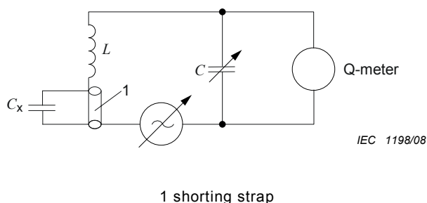
Figure 8 – Schematic diagram of the measuring circuit
