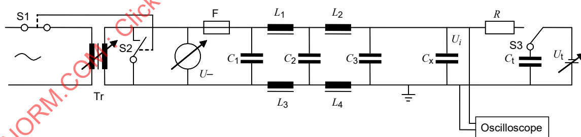
Figure 8 – Typical circuit for pulse loading of capacitors under a.c. voltage
