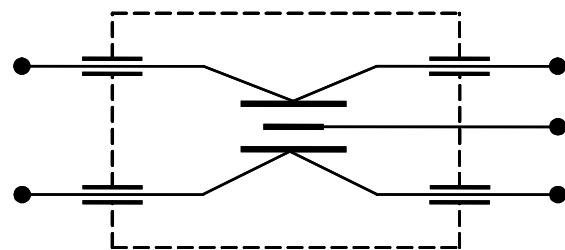
Figure 4c – Multiple unit lead-through capacitor (non-coaxial) for symmetrical and asymmetrical use
