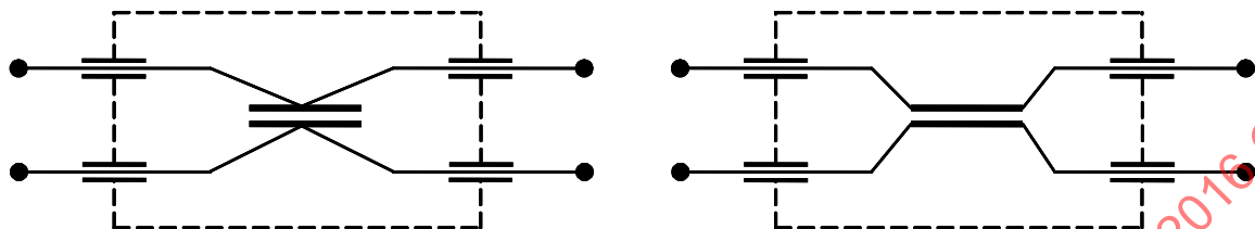
Figure 4a – Lead-through capacitor for symmetrical use (non-coaxial)
