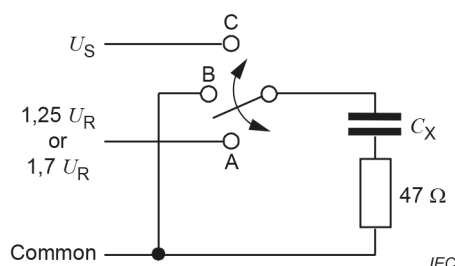
Figure B.1 – Endurance test circuit
