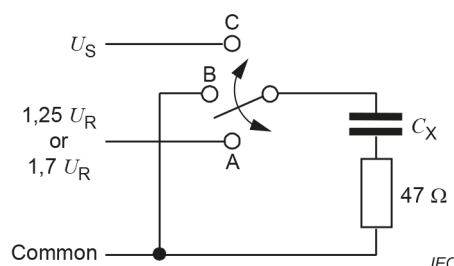
Figure B.1 – Endurance test circuit
