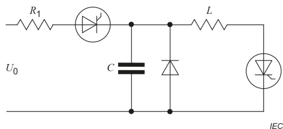
Figure E.2 – Inductive pulse test circuit
