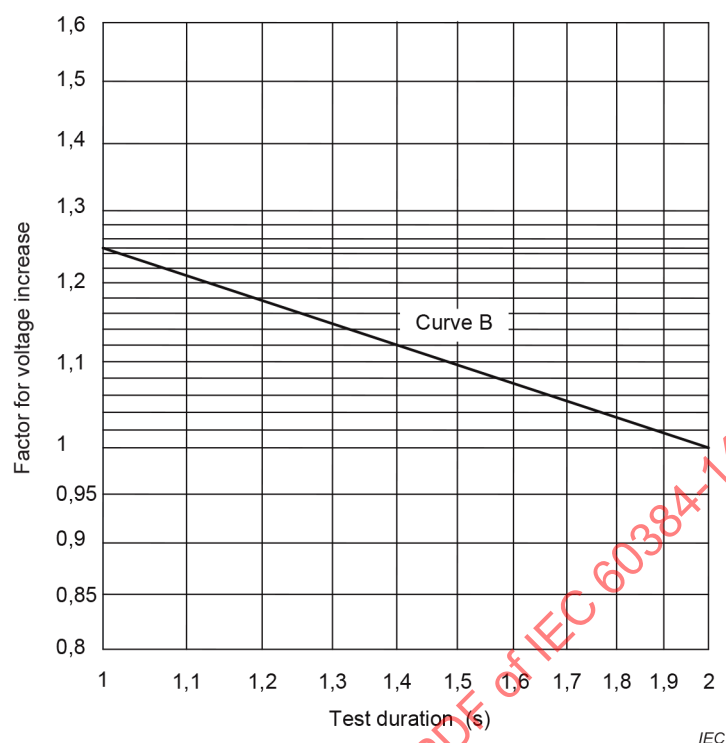
Figure 9 – Increased voltage for tests below 2 seconds
