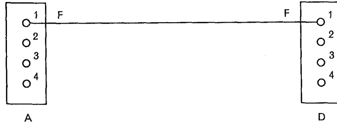
FIG. 6. — Example of functional marking.
