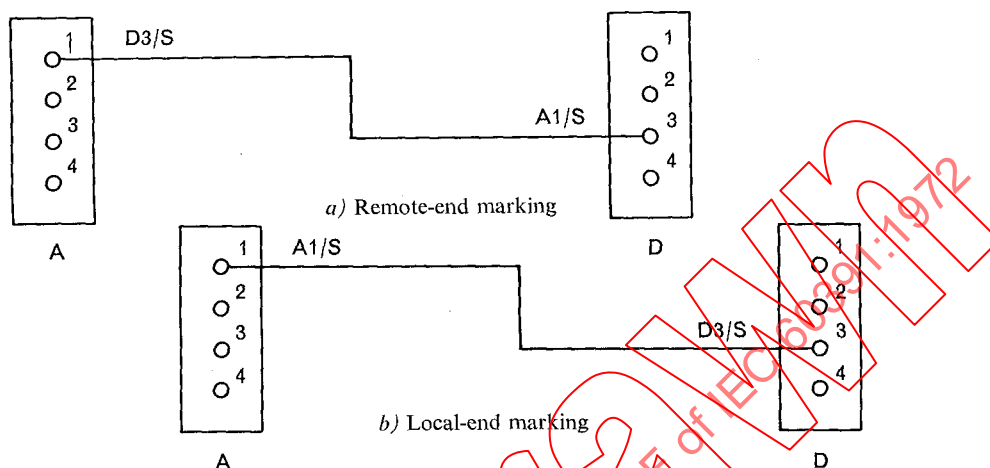
FIG. 11. — Examples of dependent marking with supplementary mark S.
