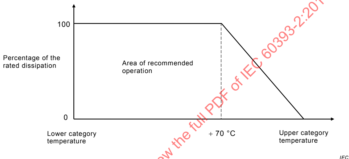
Figure 1 – Rated dissipation curve
