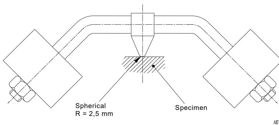
Figure 7 – Ball-pressure apparatus
