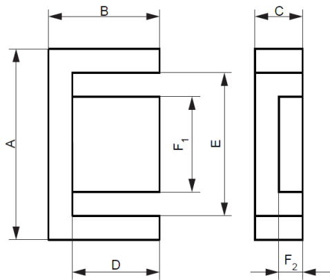
Figure 50 – EFD-core
