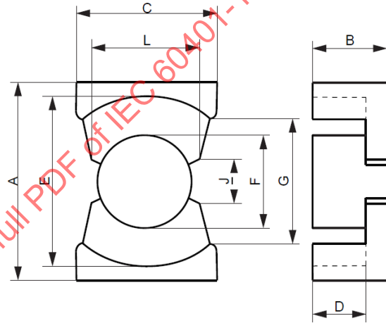
Figure 53 – PQ-core
