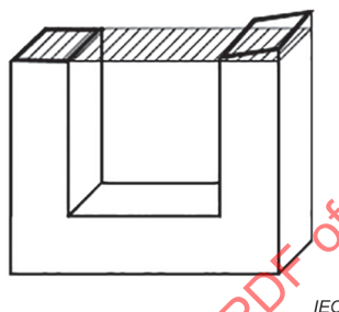
Figure 33 – Non-coplanarity
