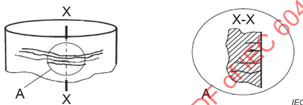
Figure 15 – Lamination
