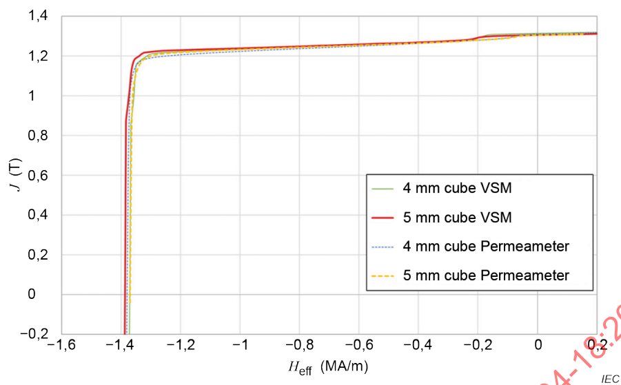
Figure E.1 – Comparison of demagnetization curves measured with a permeameter and a superconducting VSM
