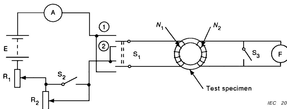
Figure 1 – Circuit for the determination of the magnetic characteristics by the ring method
