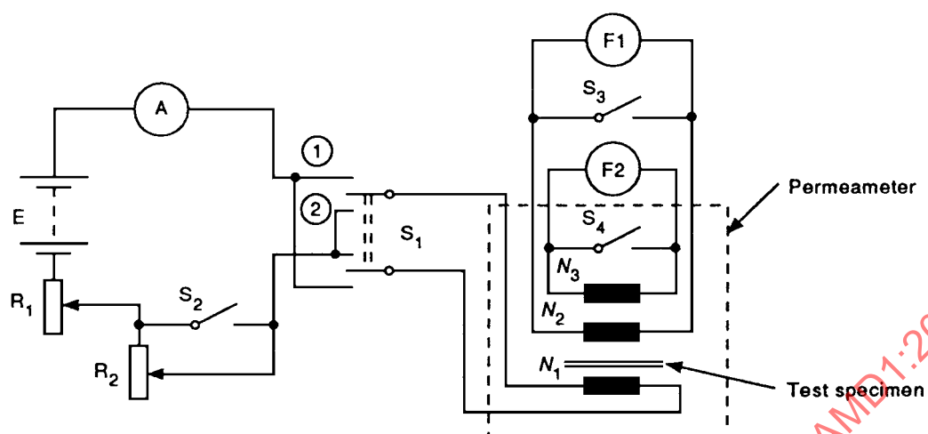
Figure 6 – Circuit for the determination of the normal magnetization curve and hysteresis loop of bar specimens using a double yoke permeameter
